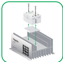
SSRP relay mounted on heat sink with thermal transfer pad (sold separately)
